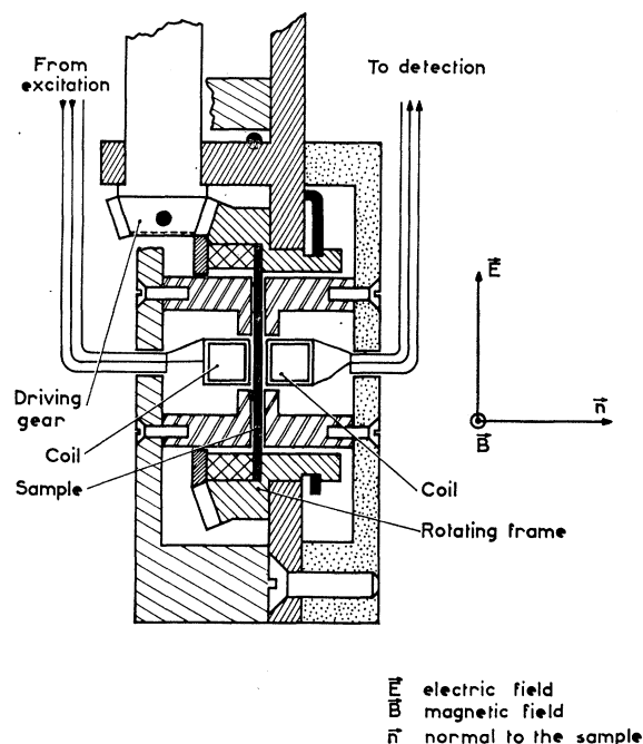
FIG. 1. Transmission setup.
